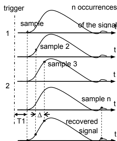
Figure 2. Sequential equivalent-time sampling.
