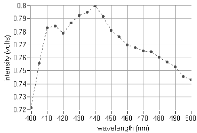
Figure 9. Florescence spectrum emitted by white color bond paper.
