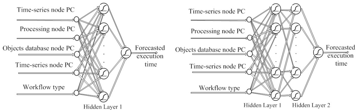
Figure 4. ANN architecture (with one and two hidden layers).
